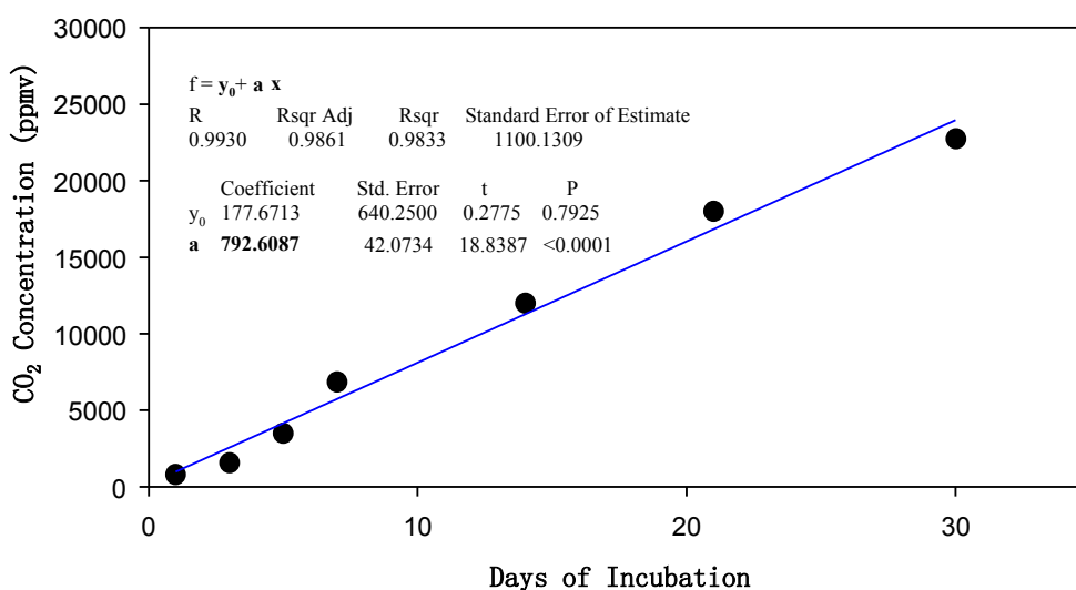
Figure 3. Example of the \text{CO}_2 accumulation in the headspace of a sample vial over the 30 day incubation period. The slope calculation is shown on the figure, which corresponds to a rate of 792.6 ppmv \text{CO}_2 \text{ day}^{-1} and by using Equation (6) a mass based production rate of 10.2 \mu\text{g-C g}^{-1} \text{day}^{-1} .
