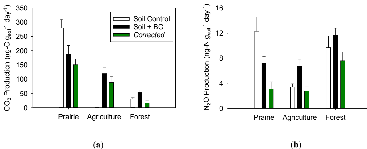
Figure 1. Average (a) CO 2 and (b) N 2 O production rates observed from the control soils, biochar amended soils, and the mathematically corrected production rates over the entire 30 day incubation period. Rates were calculated from the slope of the change in headspace concentration with time from gas samples taken at various times during the incubation (Section 4.3). The error bars represent one standard deviation.
